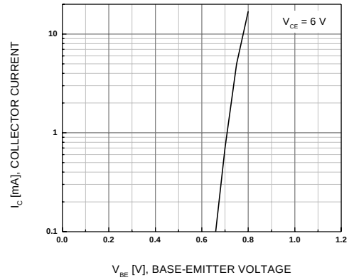
Figure 2. Base-Emitter On Voltage
