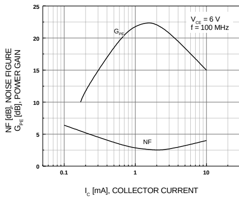
Figure 17. Power Gian & NF
