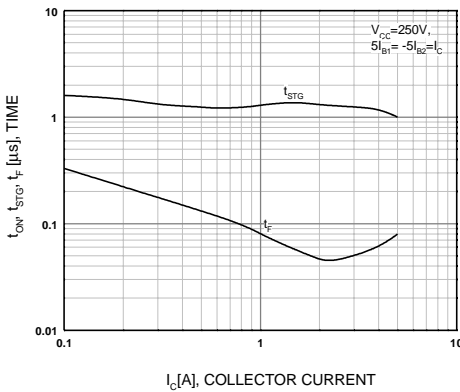
Figure 5. Switching Time
