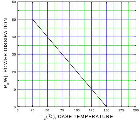
Figure 24. Power Derating
