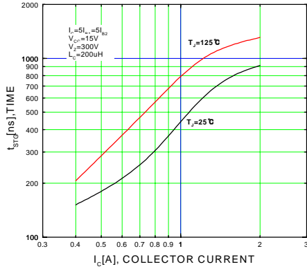
Figure 19. Inductive Switching Time, t_{STG}
