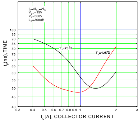
Figure 15. Inductive Switching Time, t_f
