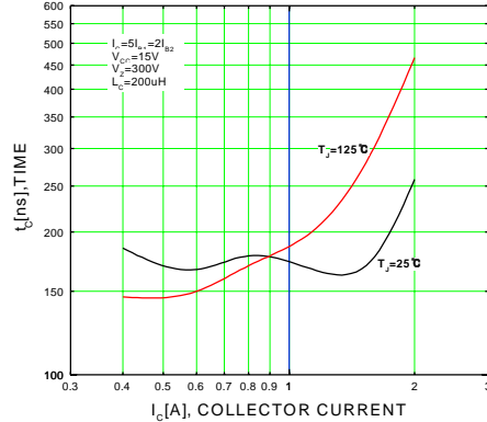
Figure 16. Inductive Switching Time, t_c
