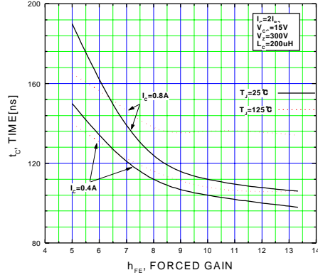
Figure 22. Inductive Switching Time, t_C
