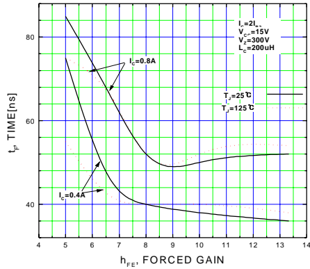
Figure 21. Inductive Switching Time, t_F
