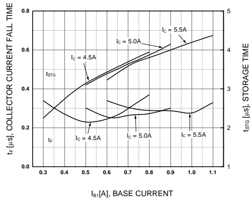
Figure 6. Switching Time
