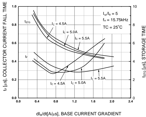
Figure 5. Switching Time
