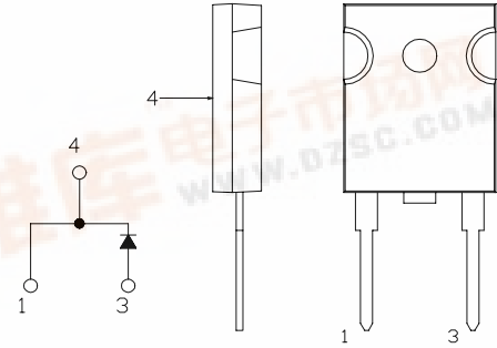
OUTLINE DRAWING
