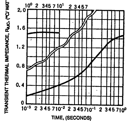
TRANSIENT THERMAL IMPEDANCE CHARACTERISTICS (DIODE)
