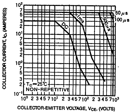
FORWARD BIAS SAFE OPERATING AREA (S.O.A.)
