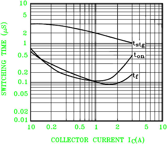
SWITCHING CHARACTERISTICS
