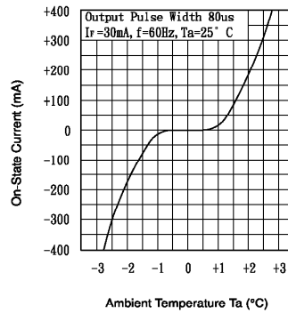
Fig.7 On-State Characteristics
