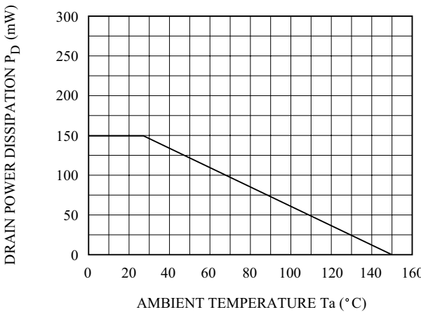
P_D - T_a
