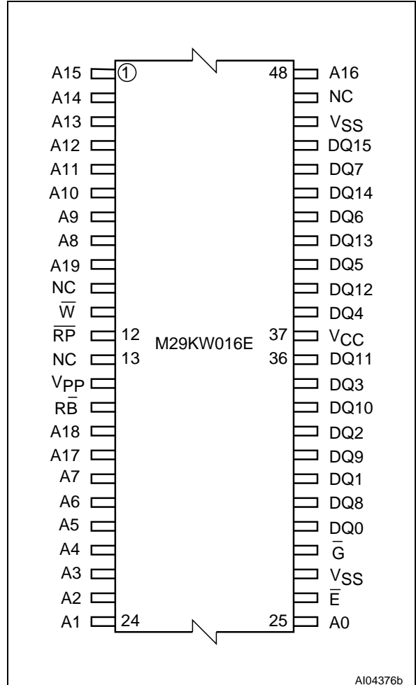
Figure 4. TSOP Connections
