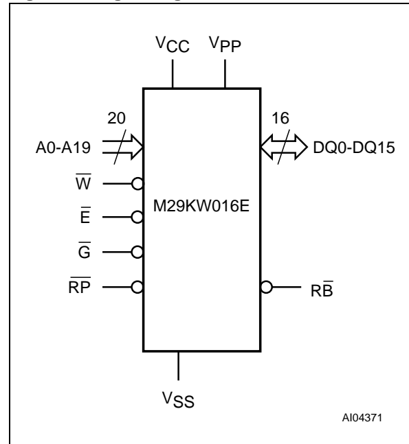
Figure 2. Logic Diagram
