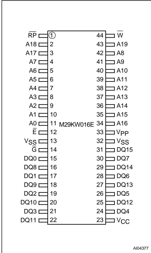
Figure 3. SO Connections
