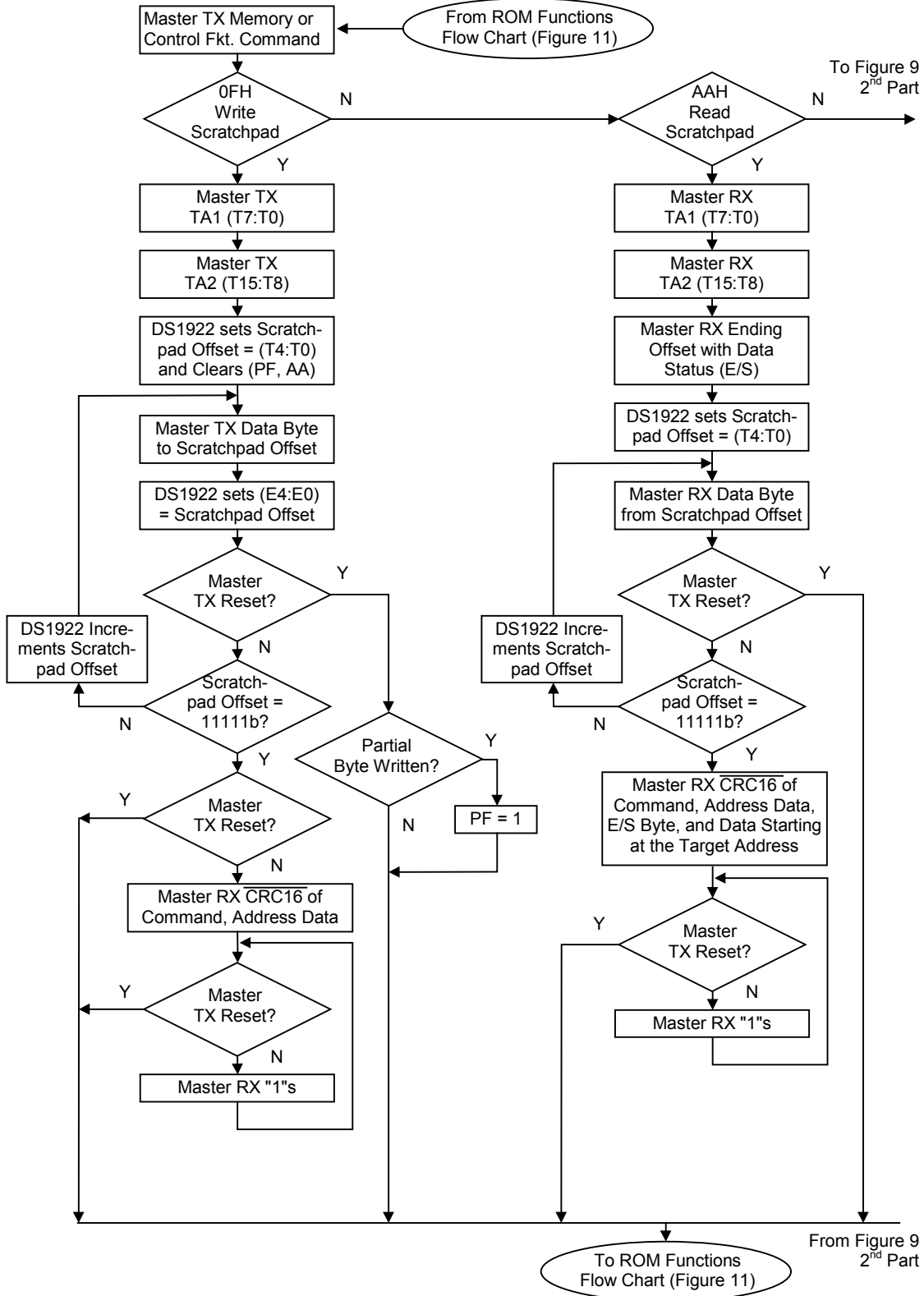
Figure 9-1. Memory/Control Function Flow Chart
