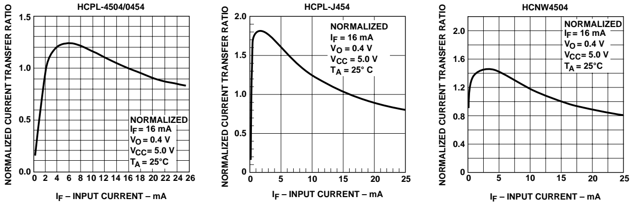
Figure 2. Current Transfer Ratio vs. Input Current.
