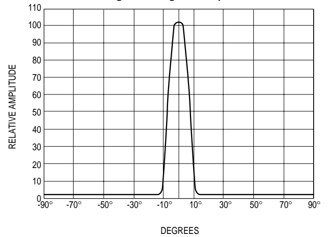
Figure 4. Angular Response
