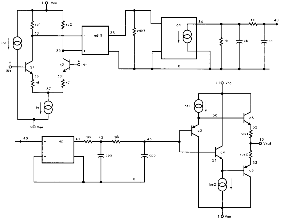
EL2190 Macromodel — Contd.
