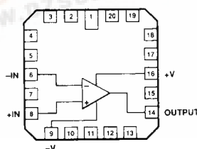
20-Lead LCC
