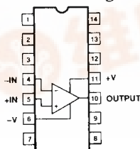
CerDIP Package
