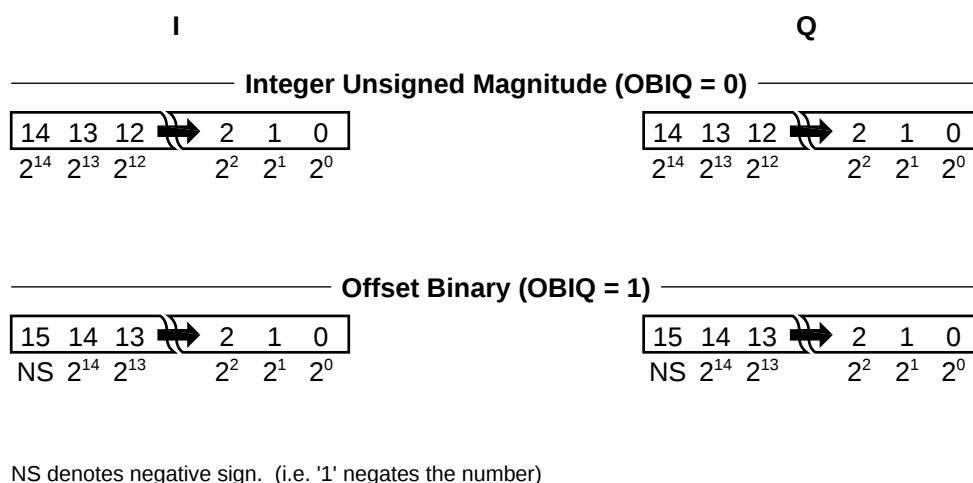
FIGURE 1B. OUTPUT FORMATS
