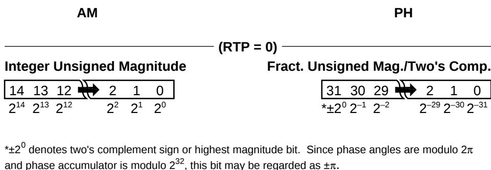
FIGURE 1A. INPUT FORMATS
