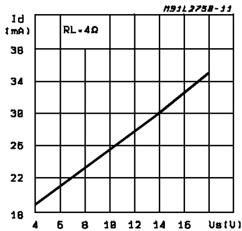
Figure 15: Quiescent Drain Current vs. Supply Voltage
