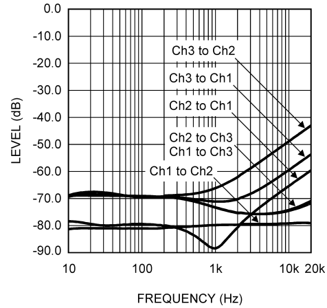
Crosstalk vs Frequency \pm 24V , P_{OUT} = 10W , R_L = 8\Omega , 80kHz BW
