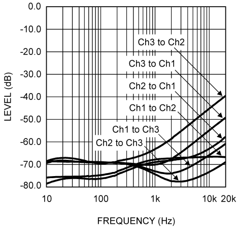
Crosstalk vs Frequency \pm 19V , P_{OUT} = 10W , R_L = 4\Omega , 80kHz BW
