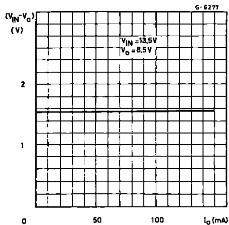
Figure 6 : Dropout versus Load Current
