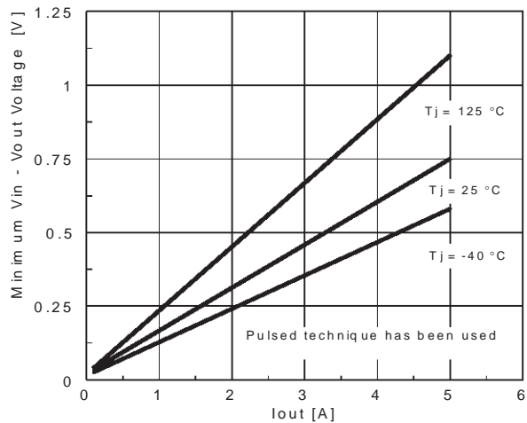
Figure 5: Dropout Voltage
