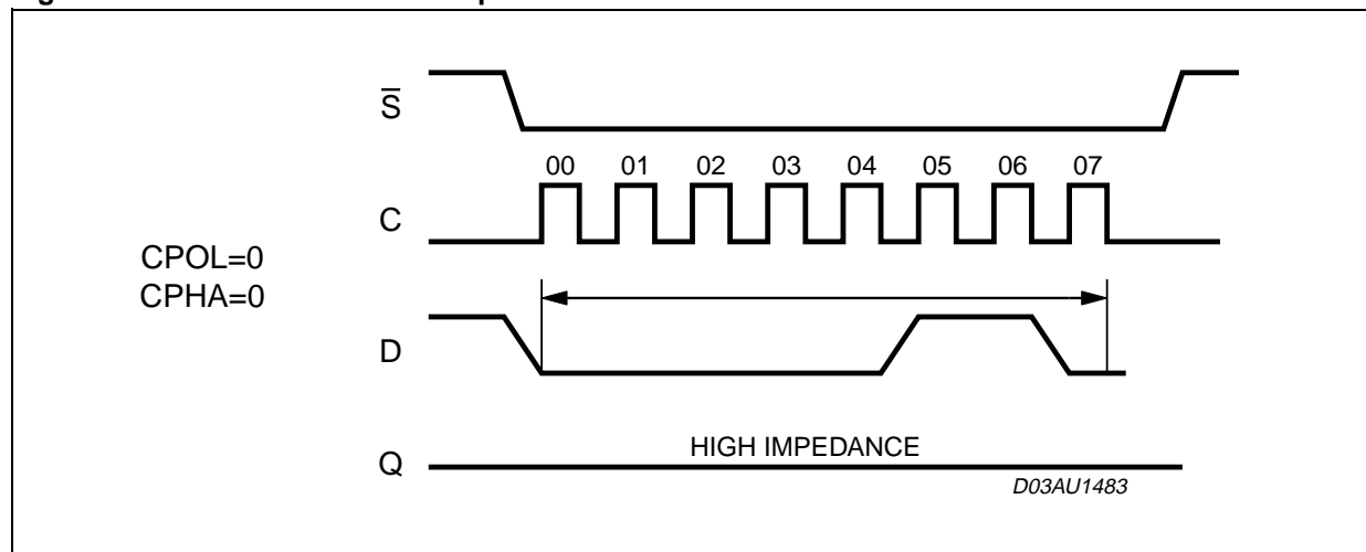
Figure 11. Write Enable Latch Sequence
