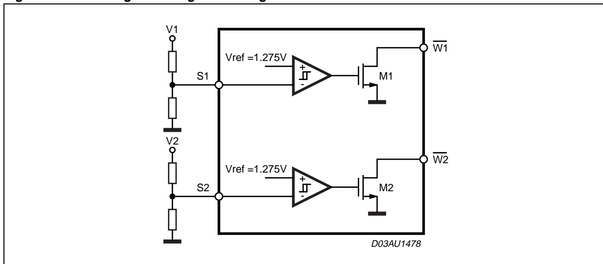
Figure 7. Low Voltage Warning Block Diagram.
