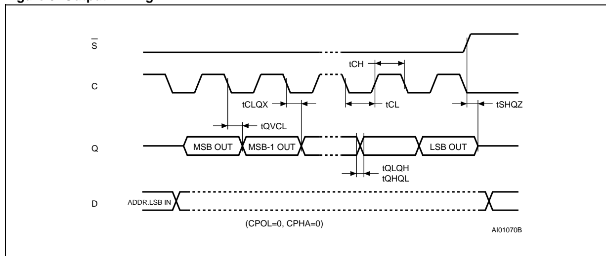
Figure 3. Output Timing
