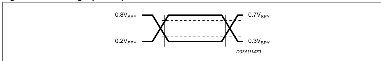
Figure 1. AC Testing Input Output Waveforms
