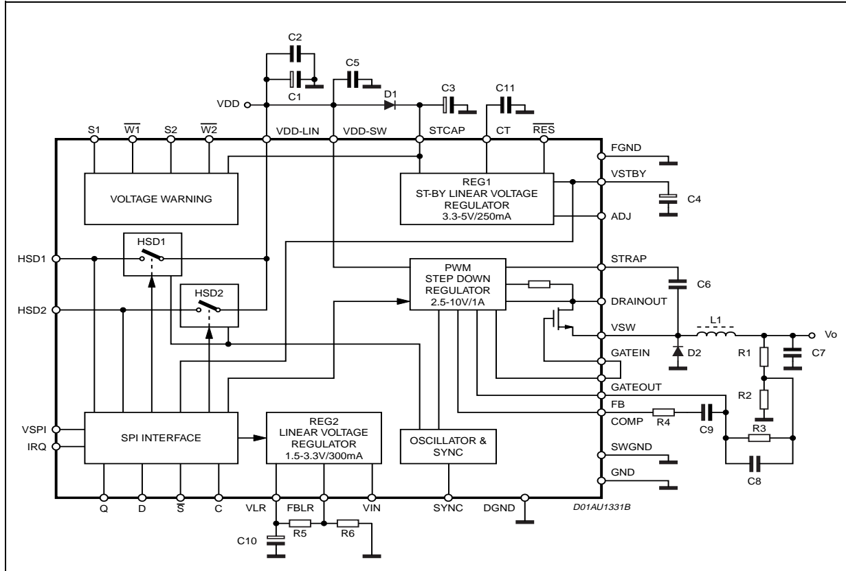
Figure 19. Block Diagram And Application With External Power MOS
