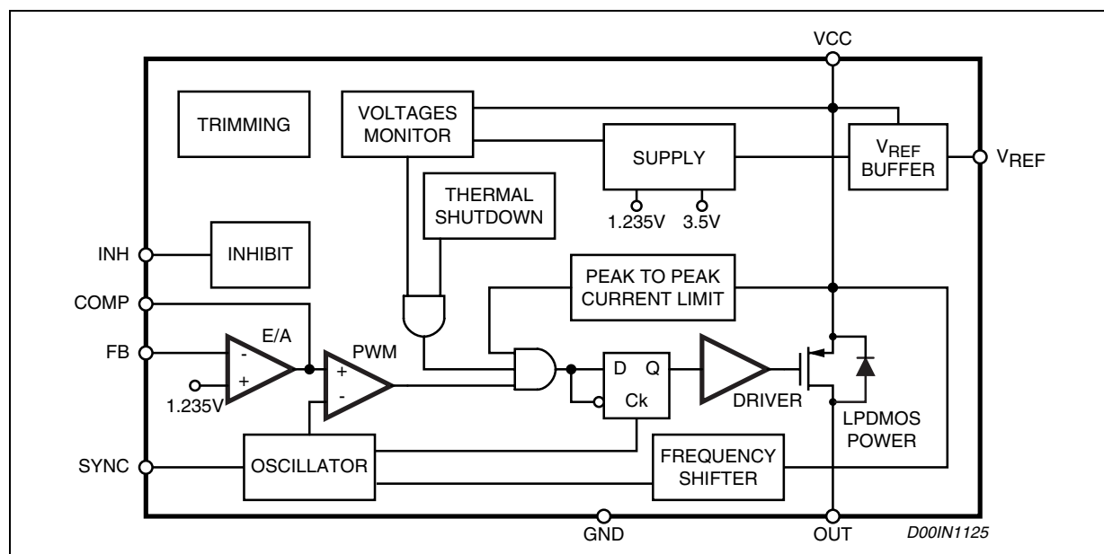
Figure 4. Block Diagram
