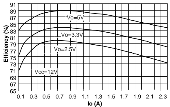
Figure 13. Efficiency vs. Output Current ( V_{CC} = 12V )
