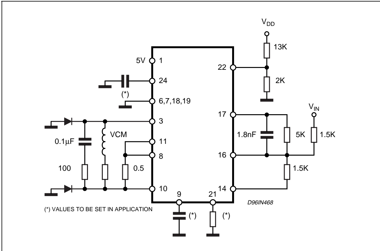
Figure 1: Application Circuit
