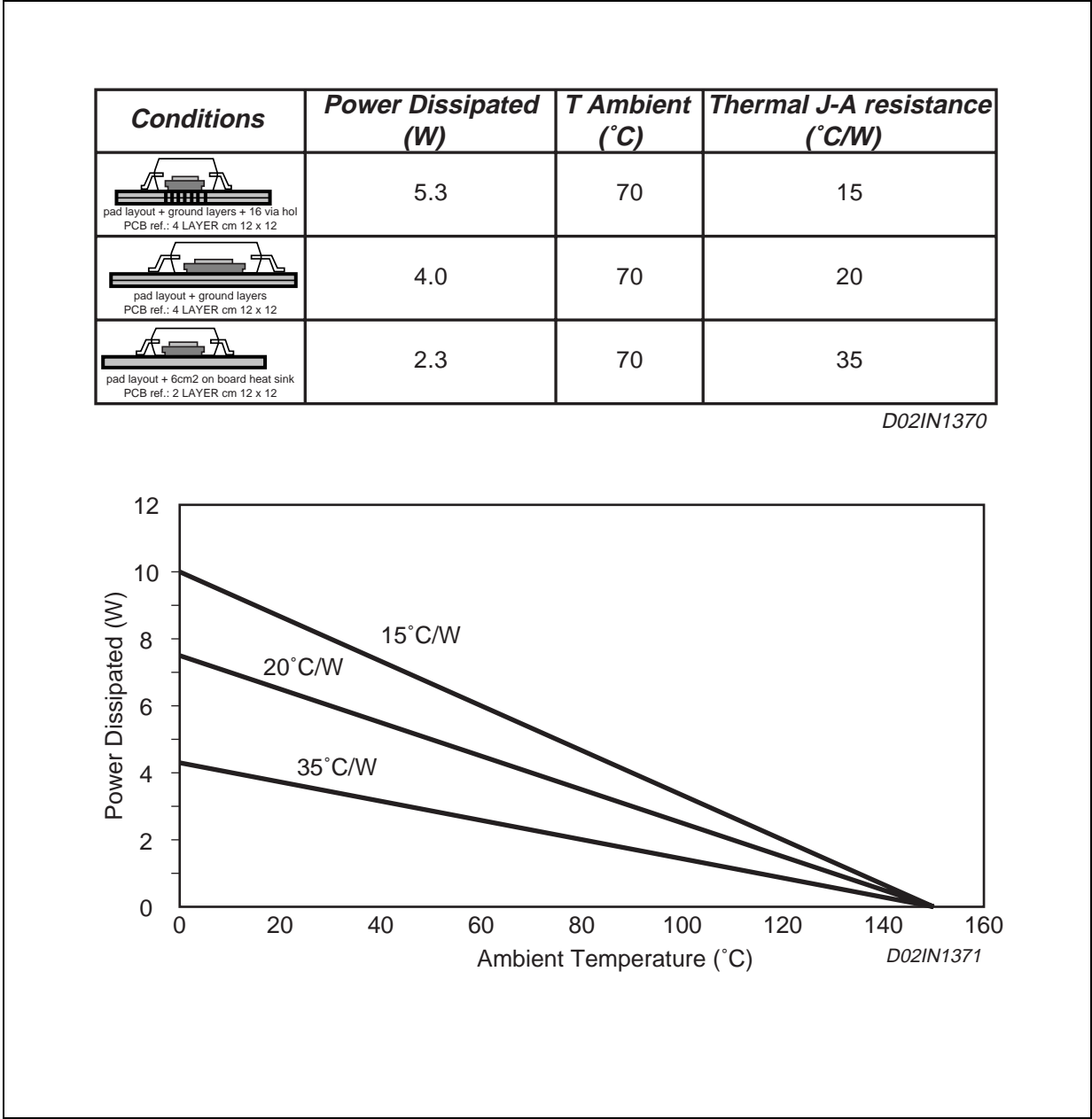
Figure 4. Thermal Characteristics
