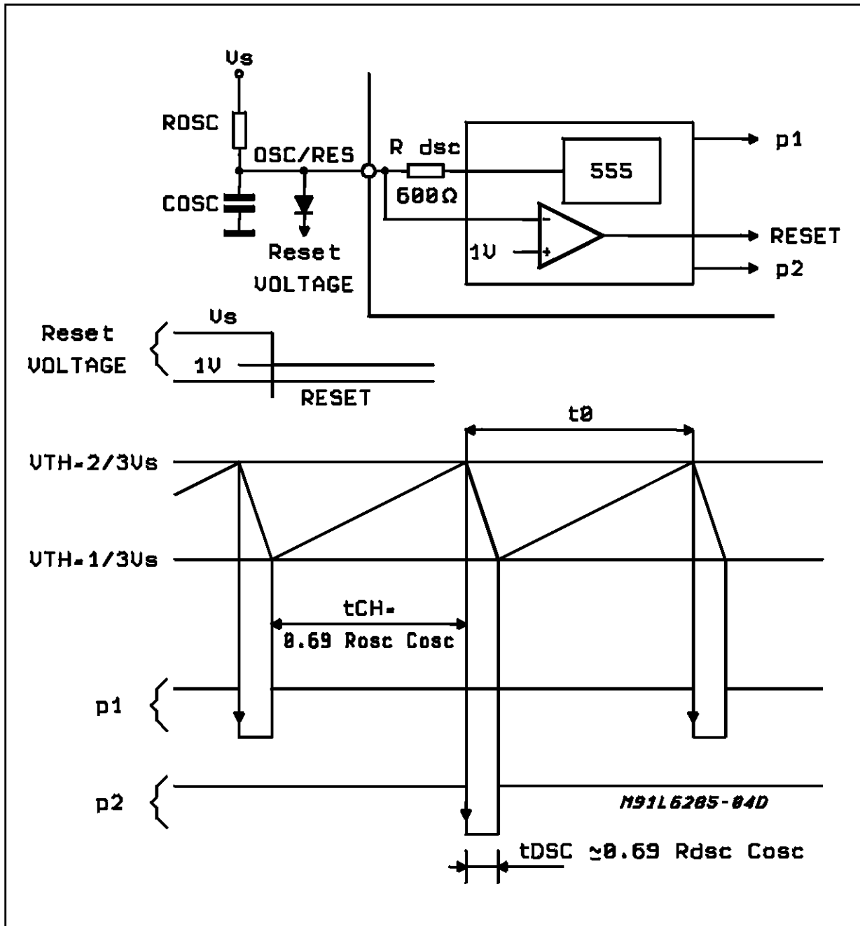
Figure 6: Oscillator Concept
