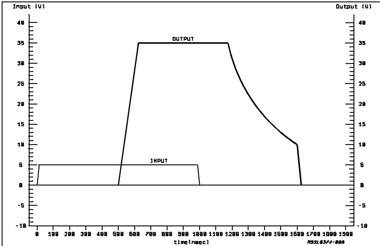
Figure 9: Switching Waveforms.
