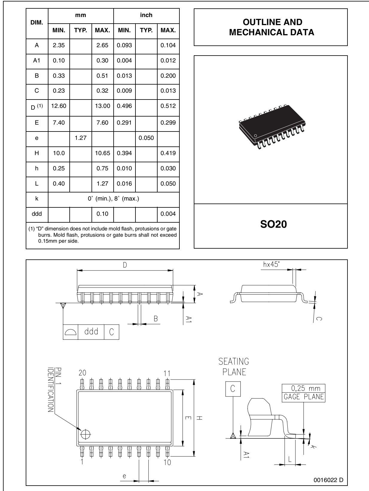
Figure 7. SO20 Mechanical Data &amp; Package Dimensions
