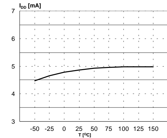
Figure 3. IC Supply current
