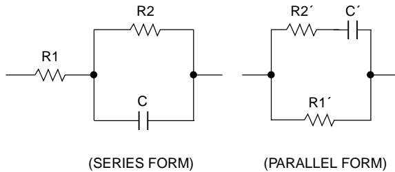
Figure 12. Equivalent Complex Terminations
