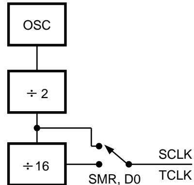
Figure 40. SCLK Circuit
