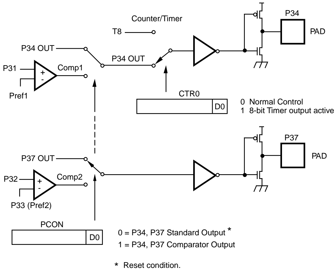
Figure 16. Port 3 Configuration
