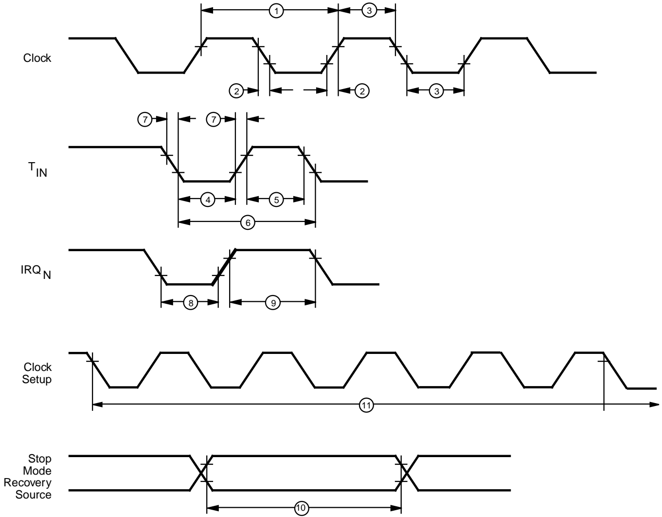
Figure 10. Additional Timing
