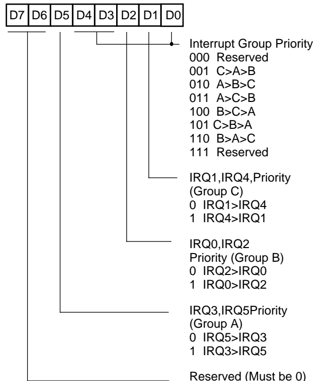
Figure 56. Interrupt Priority Registers ((0) F9H: Write Only)
