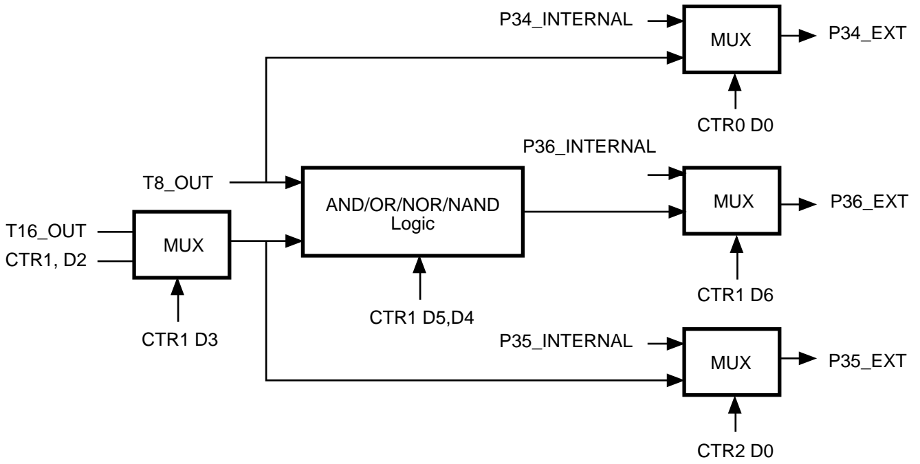
Figure 35. Output Circuit
