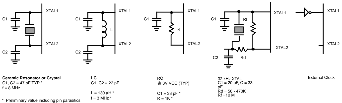
Figure 37. Oscillator Configuration
