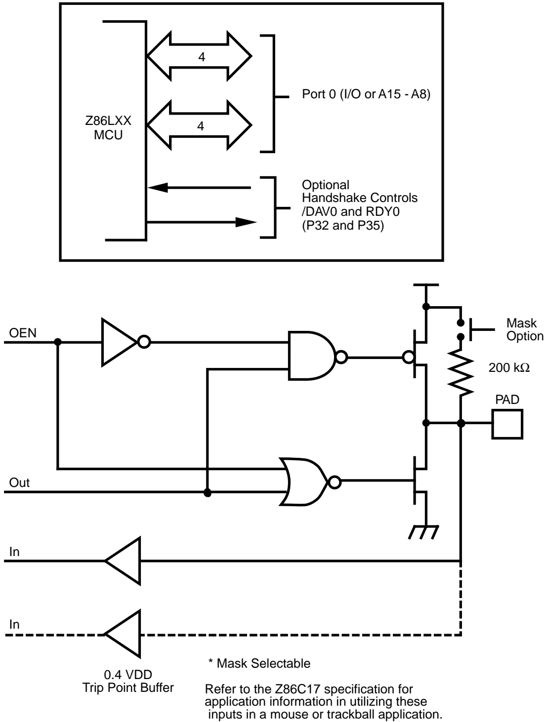
Figure 13. Port 0 Configuration
