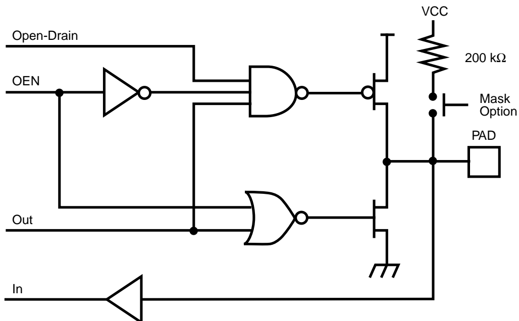
Figure 15. Port 2 Configuration
