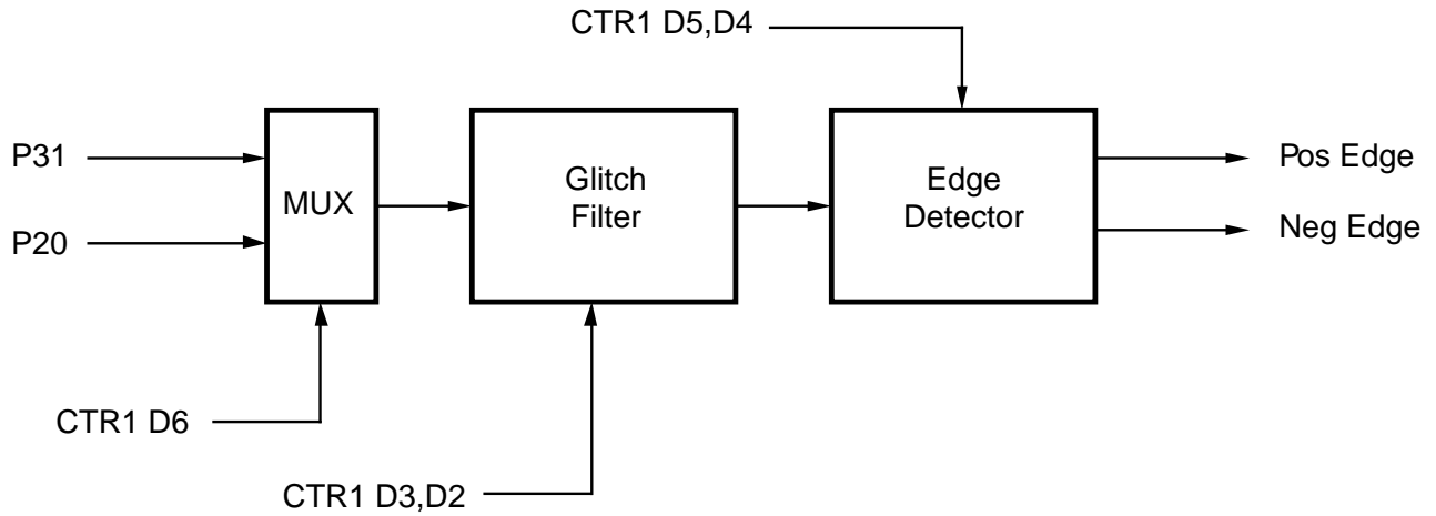
Figure 24. Glitch Filter Circuitry
