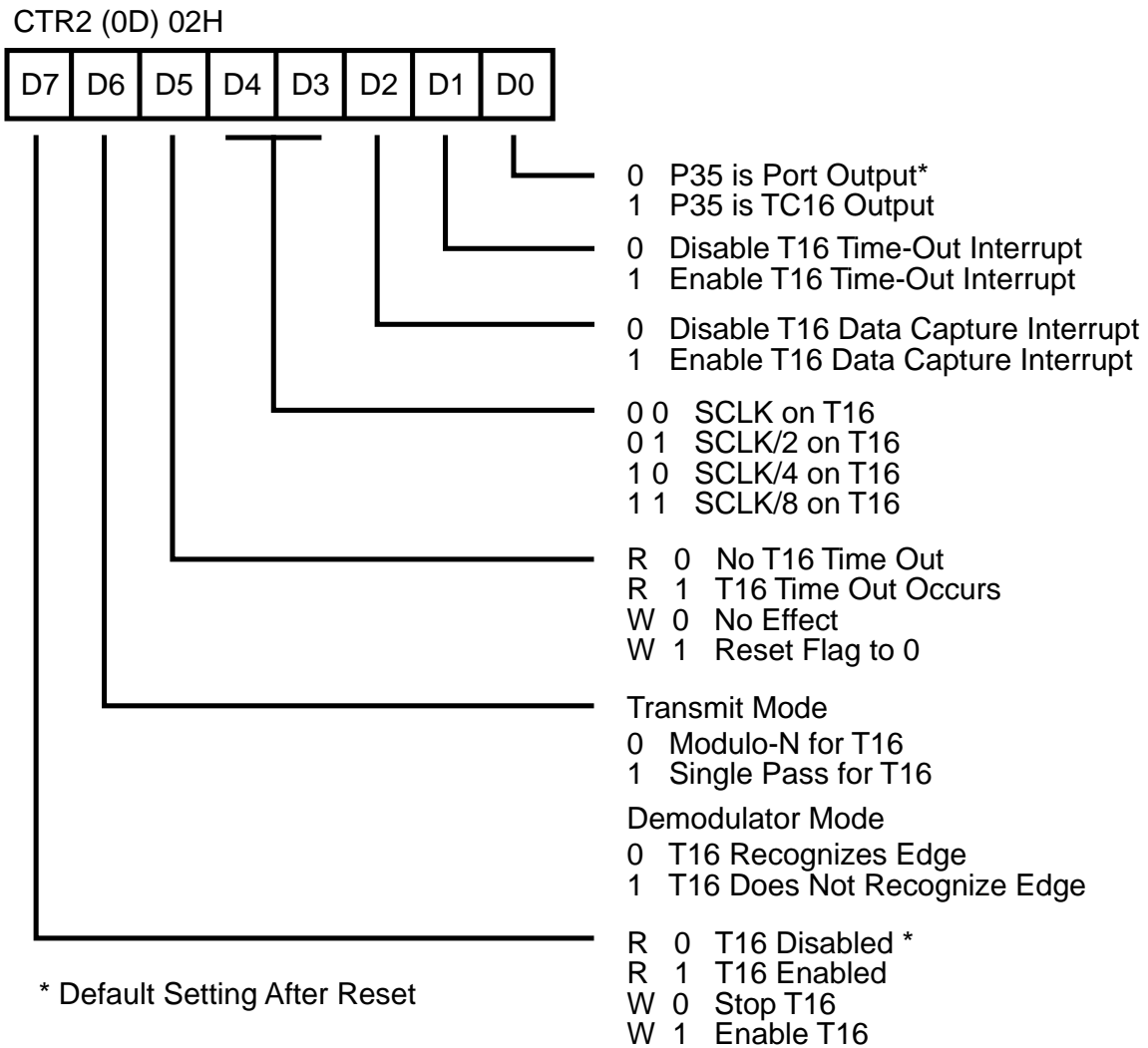
Figure 48. T16 Control Register ((0D) 2H: Read/Write Except Where Noted)
