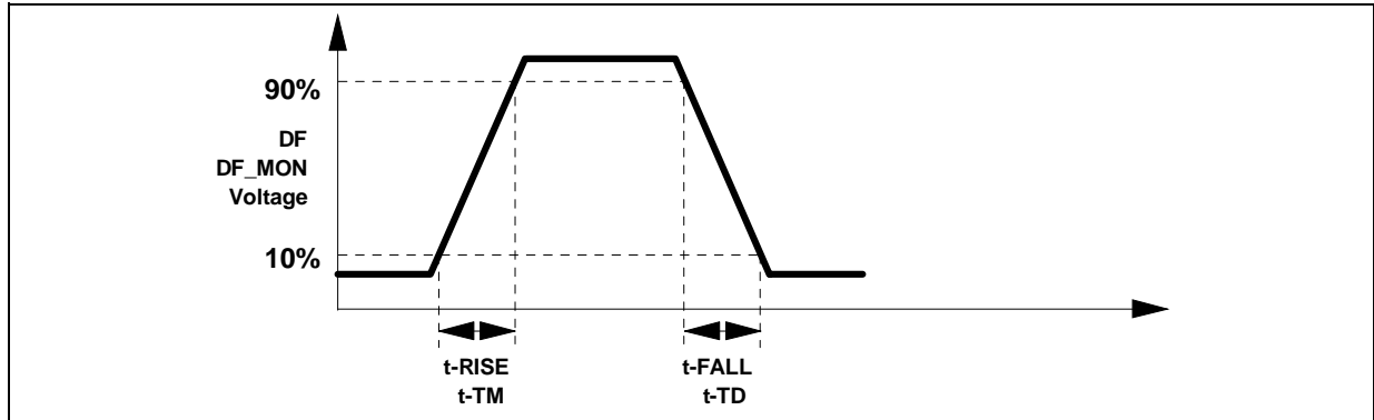
Figure 6. Output Voltage rise/fall time (DF, DF_MON)
