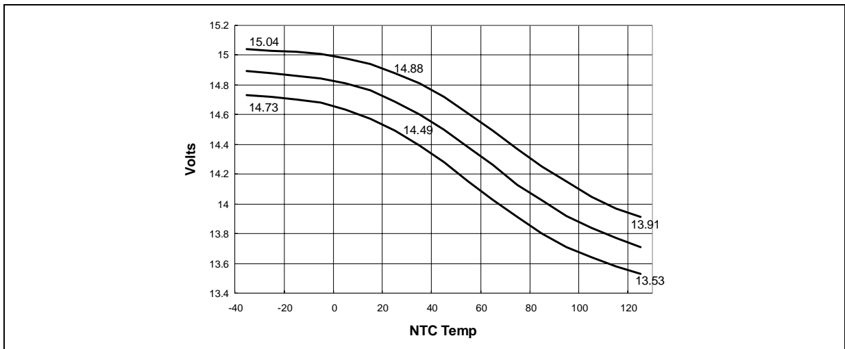
Figure 3. Set-Point Voltage vs. Thermistor Temperature, T j = 90°C (Not guaranteed by testing, depending on NTC characteristics)
