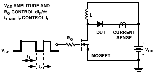
Figure 13. t_{tr} Test Circuit
