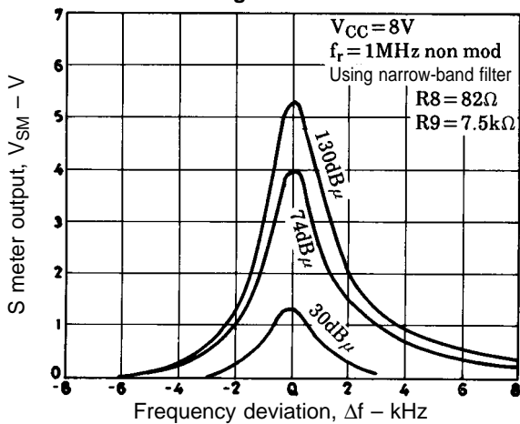
Detuning Characteristics
