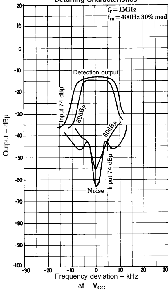
Detuning Characteristics
