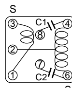
FM MIX (371DH-1108FYH)
