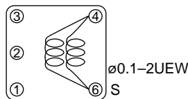
FM MIX
