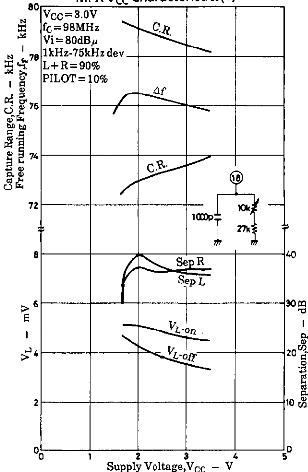
MPX VCC Characteristics(3)
