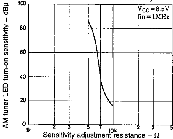
AM TU LED Turn-on Sensitivity
