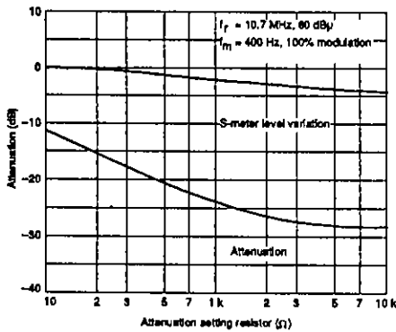
Figure 14. Muting attenuation's resistor dependence
