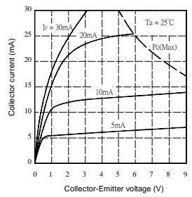
Collector current Vs. Collector-Emitter voltage
