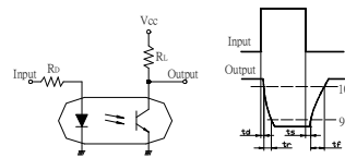
Test circuit for response time
