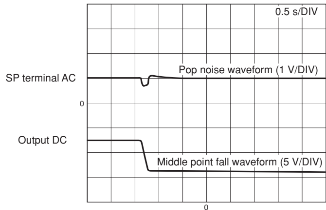
Power off output waveform
