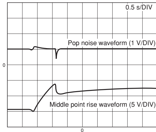
Power on output waveform
