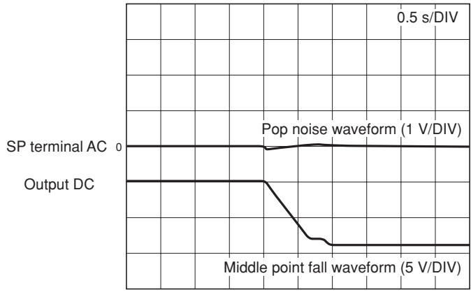
Power off output waveform ILA00960
