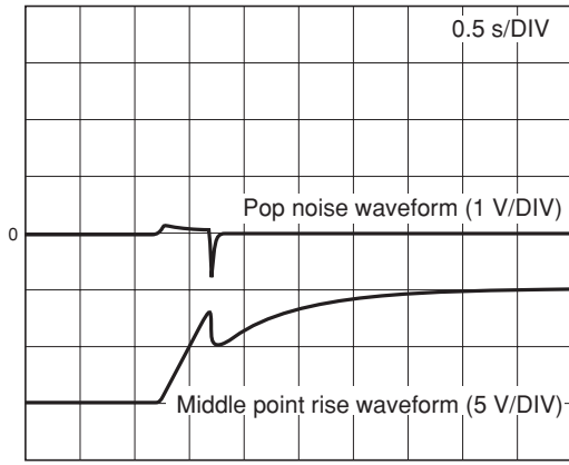
Power on output waveform ILA00959
