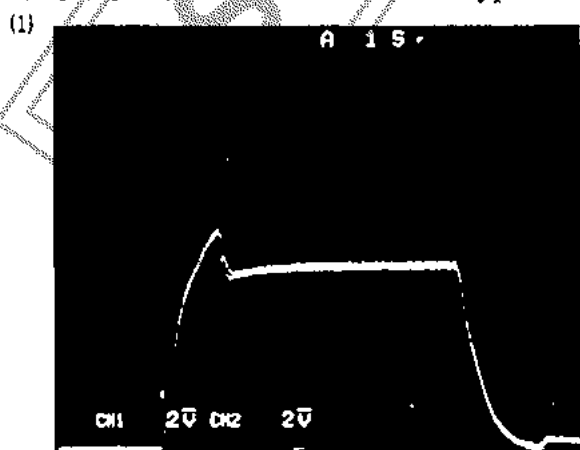
Main SW ON/OFF Characteristic of Typical Circuit ( V_{CC} = 13.2\text{V}, R_L = 4\Omega, R_g = 600\Omega )
