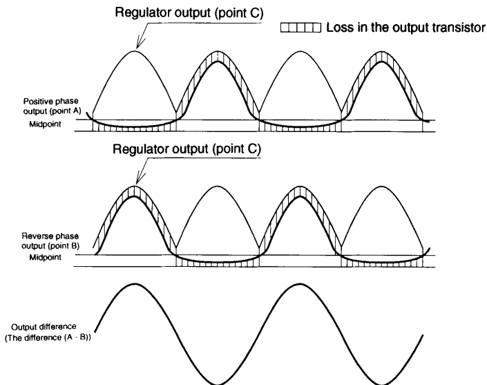
Figure 3 Output Waveforms
