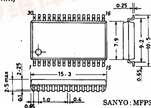
Package Dimensions 3073A-M30IC (unit : mm)
