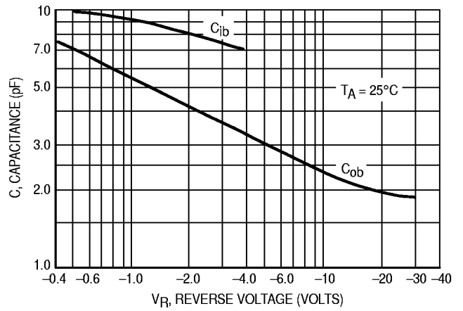
Figure 4. Capacitances
