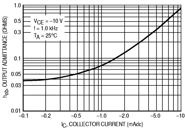
Figure 5. Output Admittance
