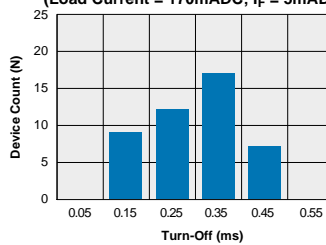
LBA127 - FormA Typical Turn-Off Time (N=50 Ambient Temperature = 25°C) (Load Current = 170mADC; I F = 5mADC)
