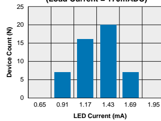
LBA127 - FormA Typical I F for Switch Operation (N=50 Ambient Temperature = 25°C) (Load Current = 170mADC)
