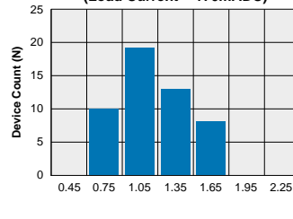
LBA127 - FormB Typical I F for Switch Dropout (N=50 Ambient Temperature = 25°C) (Load Current = 170mADC)
