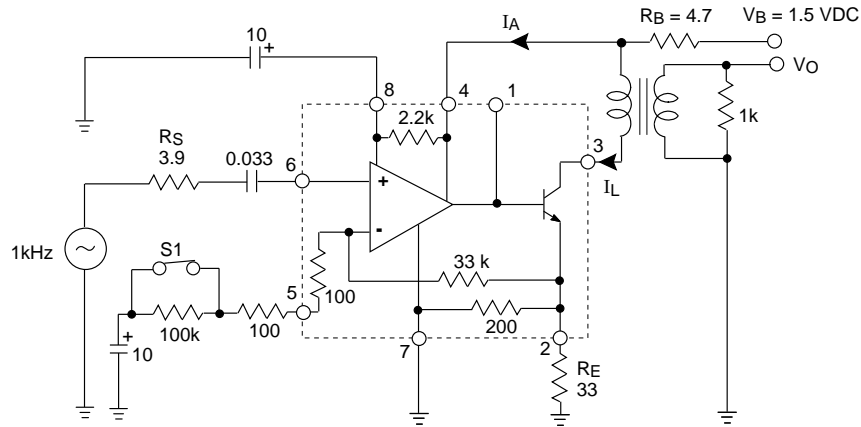
Fig. 2 LD505 Test Circuit
