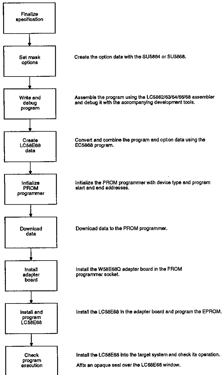
Figure 13. Development flowchart
