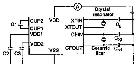
Figure 1. Supply leakage measurement
