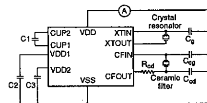
Figure 6. Supply current measurement 3
