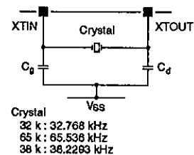
Figure 8. Crystal oscillator
