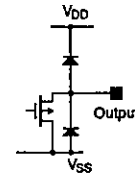
Figure 11. n-channel output
