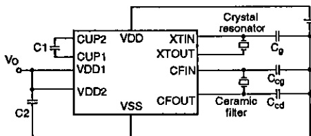
Figure 2. Output voltage measurement 1
