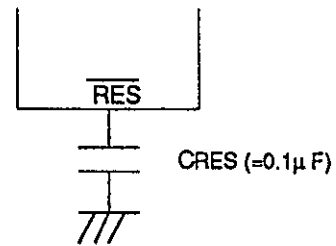
Fig. 5 Reset Circuit
