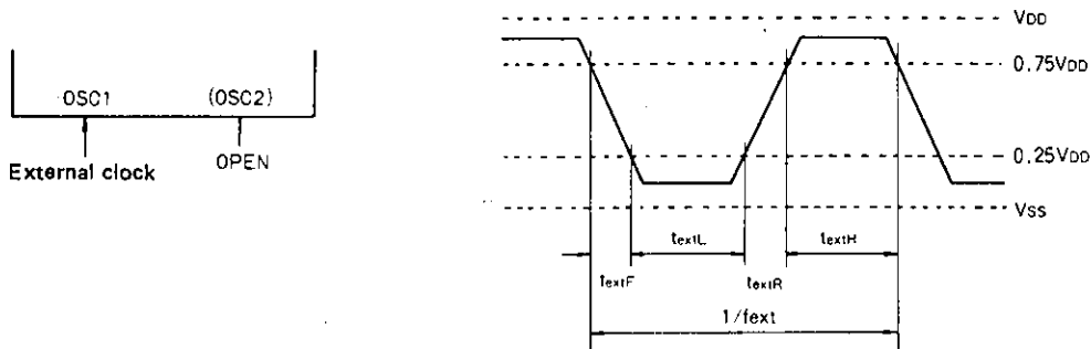
Fig. 1 External Clock Input Waveform
