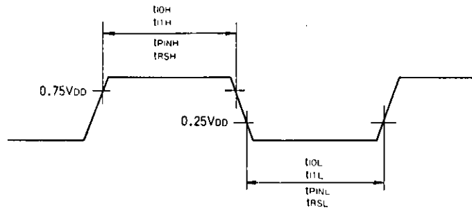
Fig. 7 INTO, INT1, INT2, PIN1, RES Input Timing
